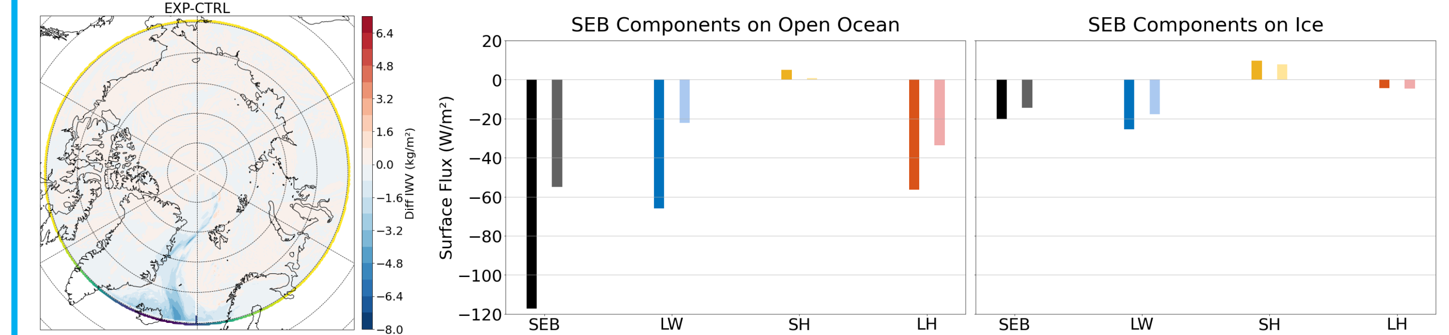
Fig. 3: Results of sensitivity run with reduced moisture inflow. Difference in IWV between experiment (EXP) and control run (CTRL) on 2019-11-16, 12 UTC (left): Colored ring at the borders show area and strength of reduction, yellow=no change, dark blue = max change of -40% inflow. Average of SEB and its component for experiment (dark colors) and control run (light colors), as in figure 2, for grid points with open ocean (center) and with sea ice (right).
