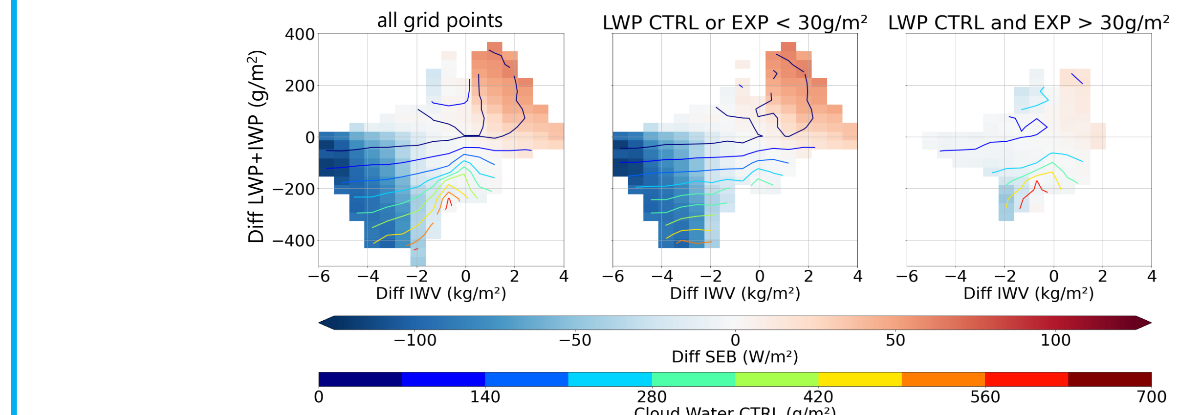
Fig. 4: Averages of differences (EXP-CTRL, including both experimental runs) in SEB, sorted by difference in IWV and sum of LWP and IWP (left), for subset of grid points where EXP or CTRL run show optically thin liquid-bearing clouds (center) and for grid points where both CTRL and EXP run show optically thick liquid-bearing clouds (right). Contour lines show the average of cloud water content of the control run in the respective bin. For threshold between optically thin and thick liquid-bearing clouds, an LWP of 30g/m 2 is used, according to the findings of Shupe and Intrieri [9].
