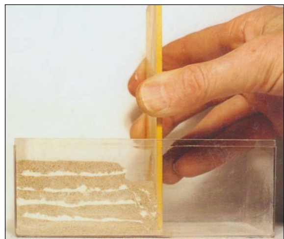
The “squeezebox” set up for tensional forces © Peter Kennett, ESEU
