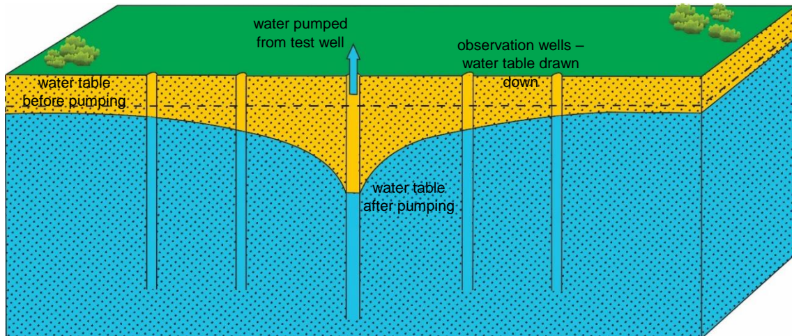
Figure 4.37. Well-testing
