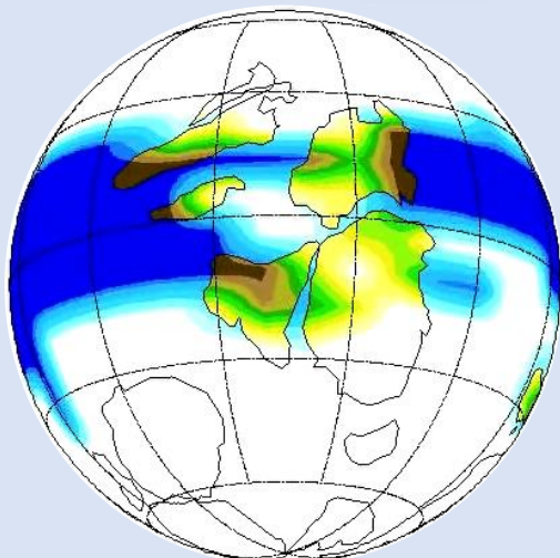
0 20 40 60 80 100 Snow and ice coverage, %
